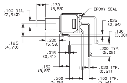
TP11 Models: omit terminal 2.
