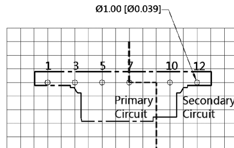
Note: Grid 2.54*2.54mm Top View PCB Layout
