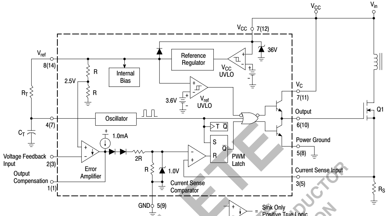
Figure 16. Representative Block Diagram
