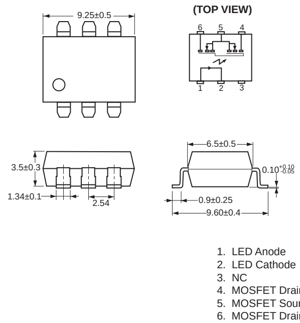
PS7122L-1A
