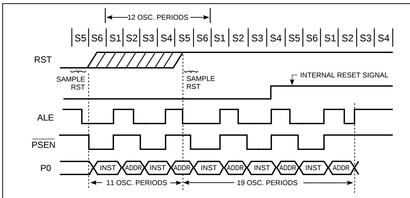
Figure 21. Reset Timing
