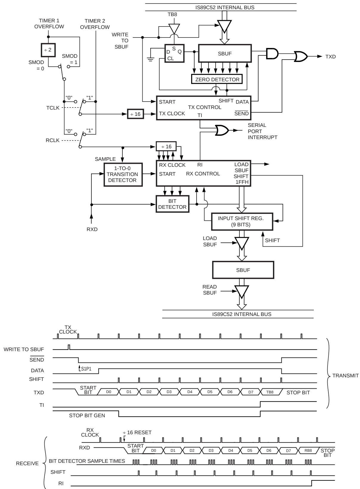
Figure 18. Serial Port Mode 3
