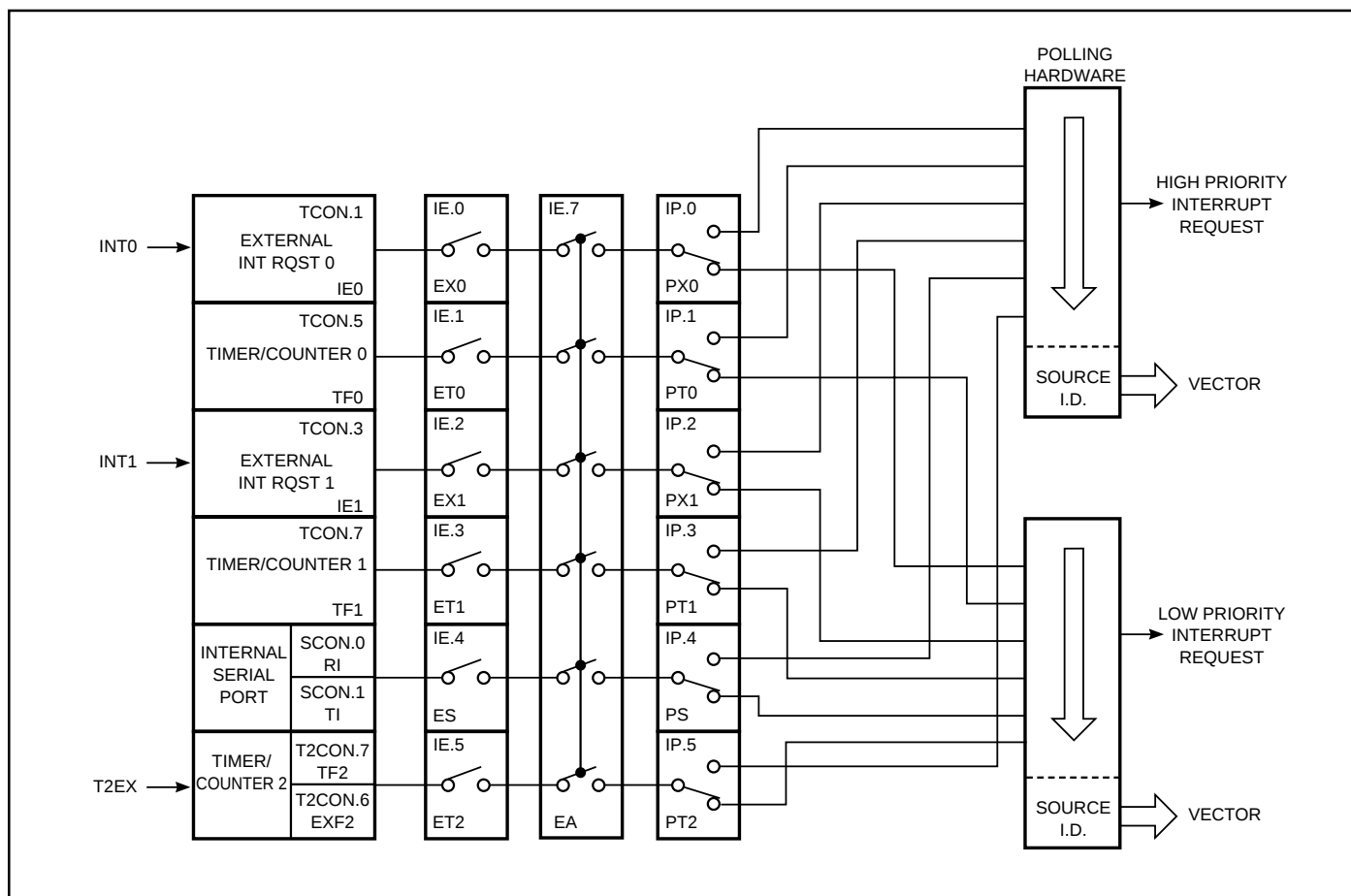
Figure 19. Interrupt System
