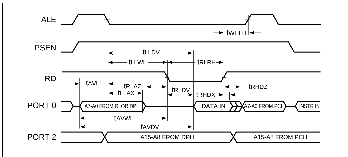
Figure 36. External Data Memory Read Cycle
