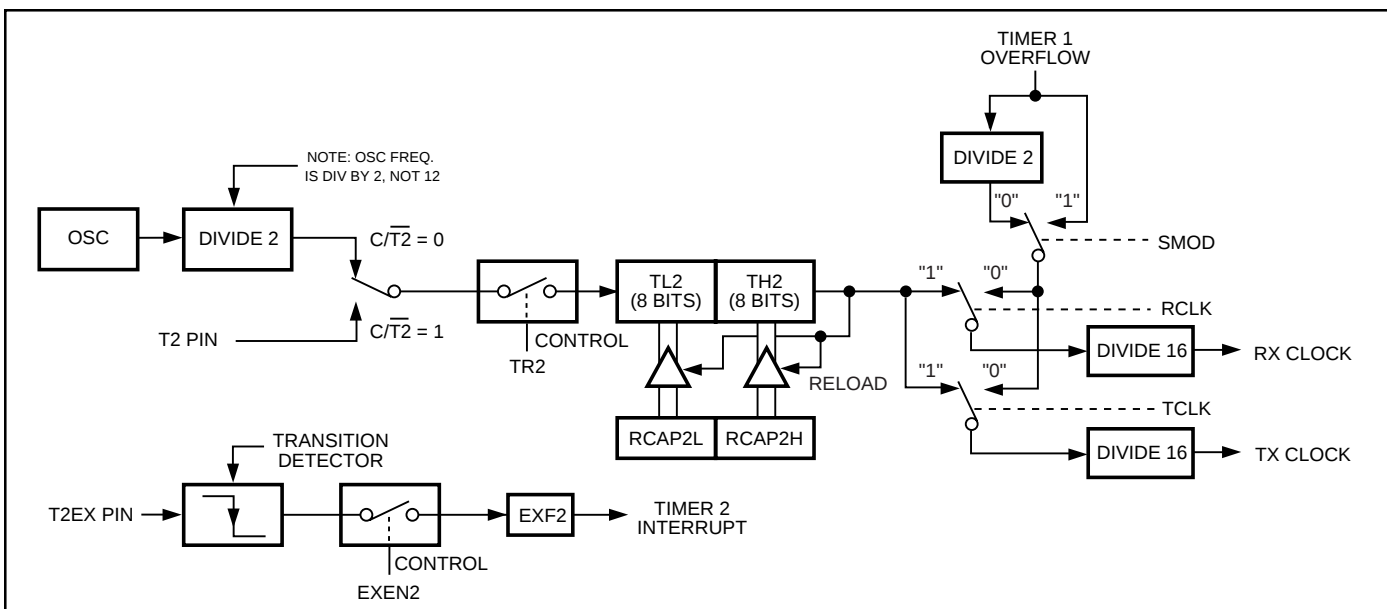
Figure 14. Timer 2 in Baud Rate Generator Mode
