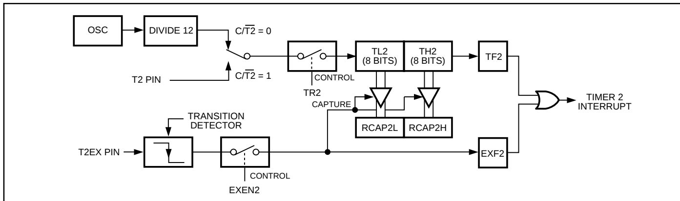
Figure 12. Timer 2 In Capture Mode
