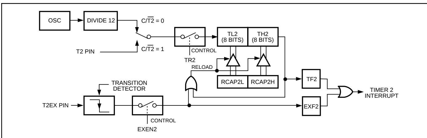
Figure 13. Timer 2 in Auto-Reload Mode
