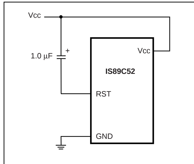
Figure 22. Power-On Reset Circuit
