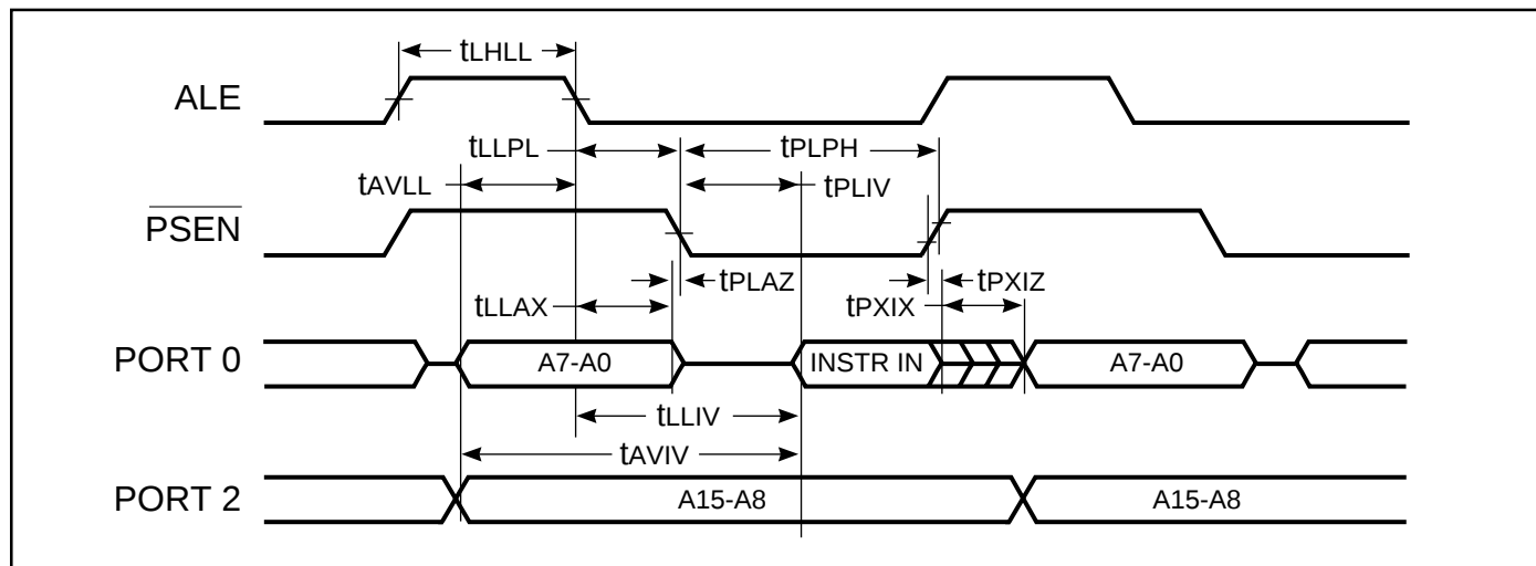
Figure 35. External Program Memory Read Cycle
