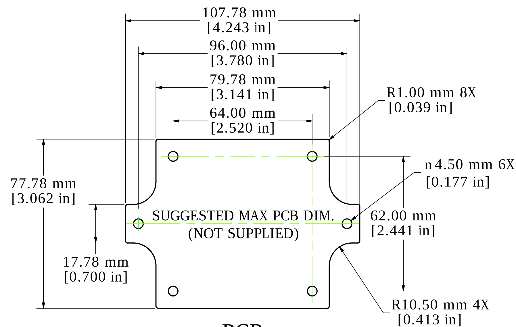
PCB
