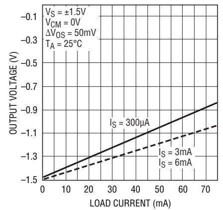
Output Voltage Swing vs I_{LOAD}
