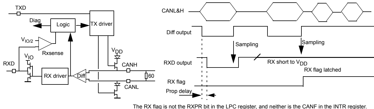
Figure 15. RX Path Simplified Schematic, Rx Short to V_{DD} Detection
