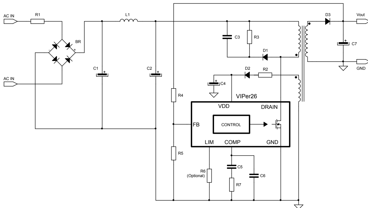
Figure 23. Flyback converter (non isolated, V_{OUT} < V_{DDCSon} )
