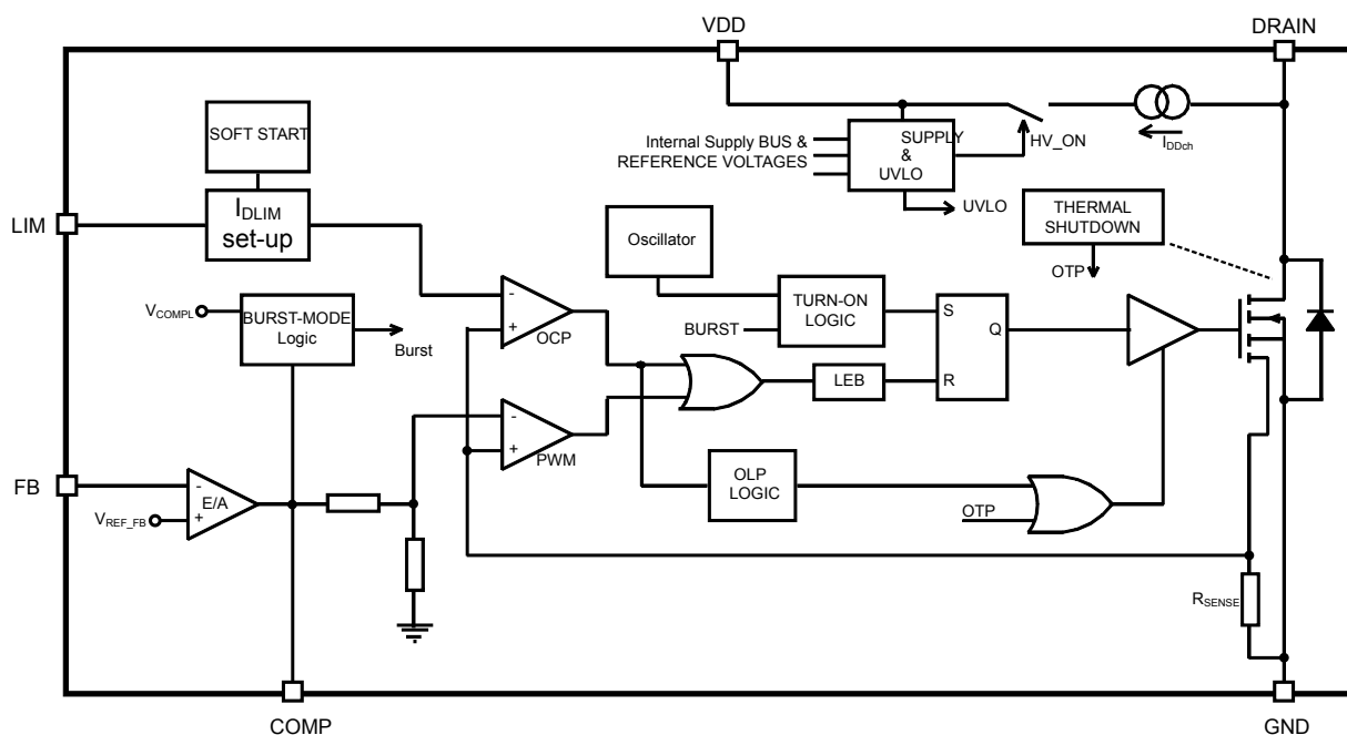
Figure 24. Block diagram
