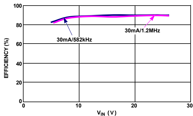
FIGURE 5. EFFICIENCY vs V_{IN} vs SWITCHING FREQUENCY AT 30mA for 4P10S (100% LED DUTY CYCLE)
