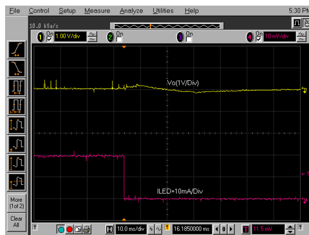
FIGURE 17. LOAD REGULATION WITH I_{LED} CHANGE FROM 100% TO 0% PWM DIMMING, V_{IN} = 12V , 4P12S AT 20mA/CHANNEL
