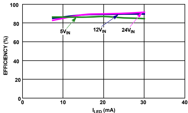
FIGURE 3. EFFICIENCY vs 30mA LED CURRENT (100% LED DUTY CYCLE) for 4P10S vs V_{IN}
