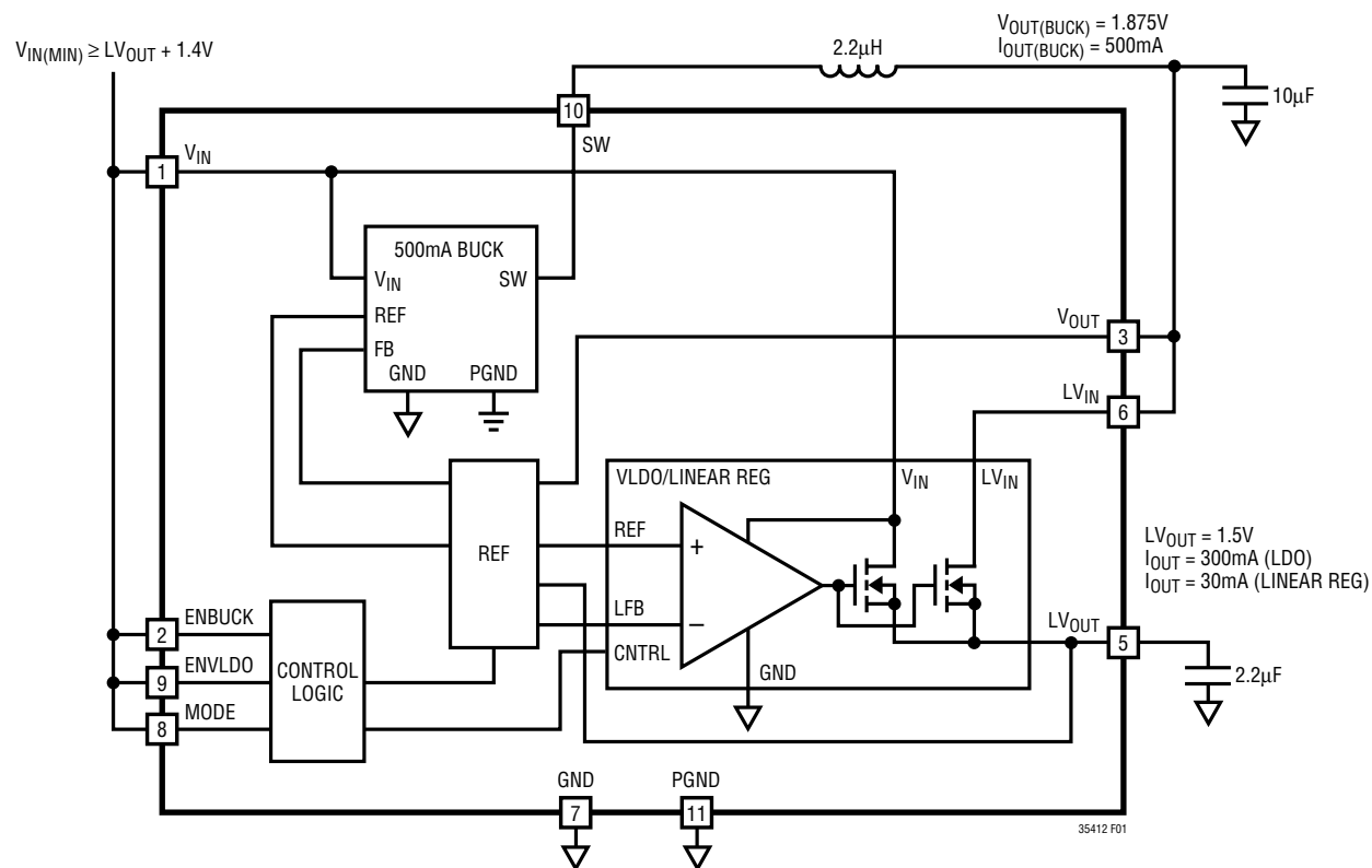
Figure 1. LTC3541-2 Functional Block Diagram
