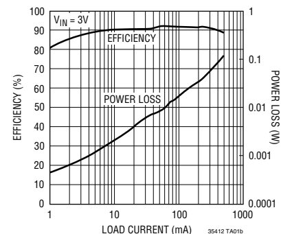
Buck (Burst) Efficiency vs Load Current
