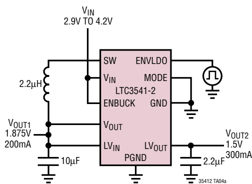
Dual Output Using Minimal External Components with V_{OUT2} Controlled by External Logic Signal, Buck in Burst Mode Operation for High Efficiency Down to Low Load Currents
