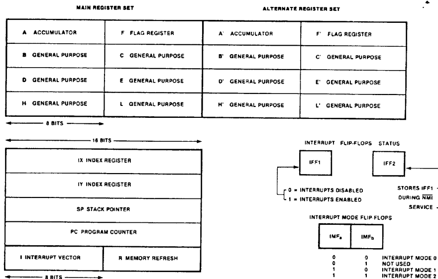
Fig. 4. CPU Registers
