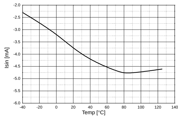
Figure 19. Output Sink Current
