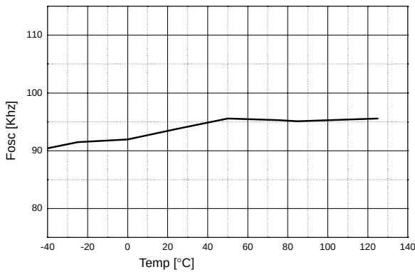
Figure 9. Oscillation Frequency (main)
