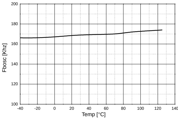
Figure 10. Oscillation Frequency (Burst)
