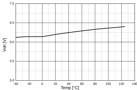
Figure 11. Output High Voltage
