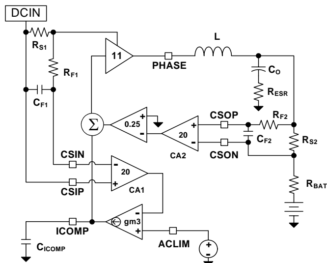
FIGURE 27. ADAPTER CURRENT LIMIT LOOP
