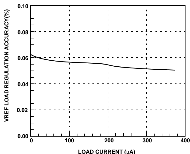
FIGURE 2. VREF LOAD REGULATION
