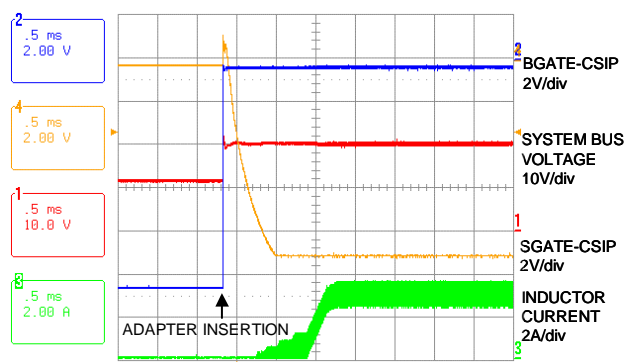
FIGURE 12. ADAPTER INSERTION
