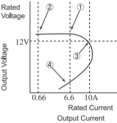
Fig2. Output Voltage/Current
