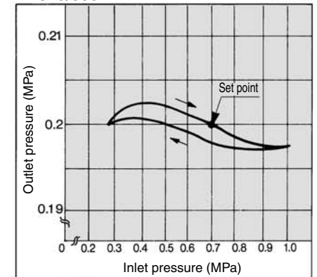
AR925/935 R_c 2
