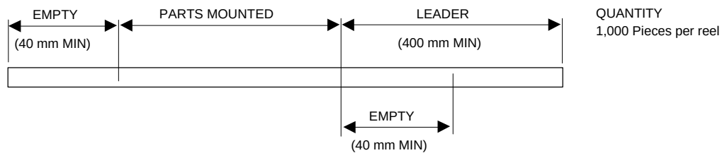
Figure 8. ZHX1010 Tape Dimensions and Configuration (Unit: mm)
