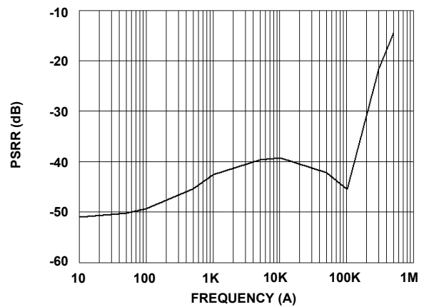
FIGURE 10. LDO1 POWER SUPPLY REJECTION ( I_{OUT1} = 100mA , C_{OUT} = 10\mu F CERAMIC)
