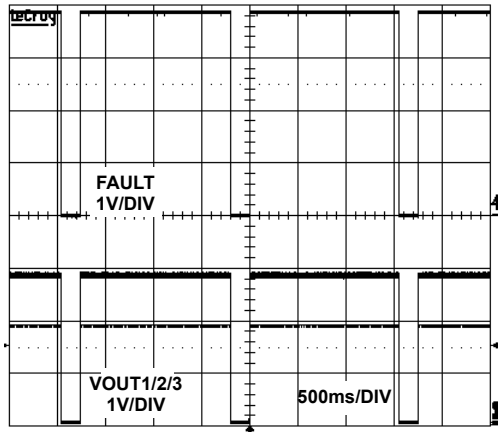
FIGURE 9. THERMAL SHUTDOWN OPERATION
