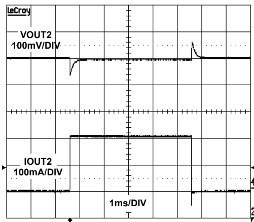
FIGURE 4. LDO2 LOAD TRANSIENT RESPONSE (10mA to 200mA)
