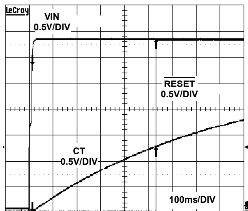
FIGURE 8. RESET DELAY DURING START-UP (CT = 0.1 \mu F )
