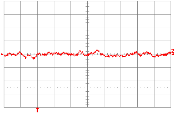
Fig. 2.0V.12: Input reflected ripple current, i_s (10 mA/div), measured through 10 \mu H at the source at full rated load current and V_{in} = 48 V. Refer to Fig. 2.0V.11 for test setup. Time scale: 1 \mu s/div.
