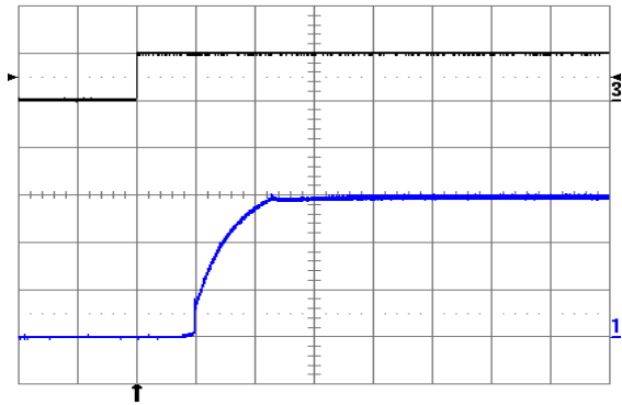
Fig. 1.5V.8: Turn-on transient at full rated load current (resistive) plus 40,000 \mu\text{F} at V_{in} = 48\text{ V} , triggered via ON/OFF pin. Top trace: ON/OFF signal (5 V/div.). Bottom trace: output voltage (1 V/div.) Time scale: 2 ms/div.
