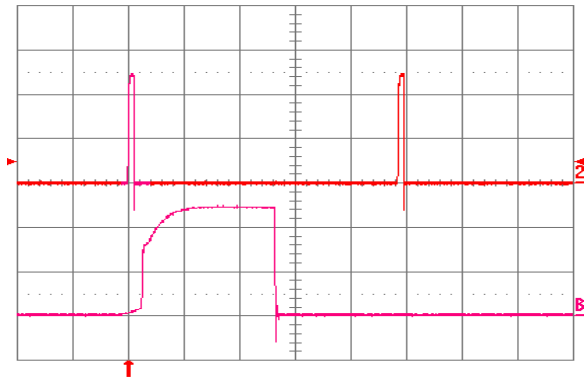
Fig. 2.0V.15: Load current (top trace, 20 A/div, 20 ms/div) into a 10 m \Omega short circuit during restart, at V_{in} = 48 V. Bottom trace (20 A/div, 1 ms/div) is an expansion of the on-time portion of the top trace.
