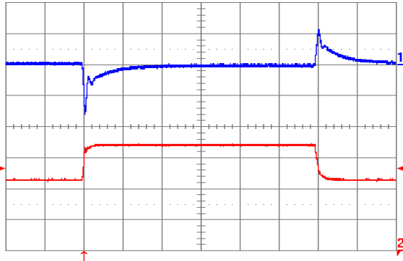
Fig. 1.8V.9: Output voltage response to load current step-change (22.5 A – 33.75 A – 22.5 A) at V_{in} = 48 V. Top trace: output voltage (100 mV/div.). Bottom trace: load current (10 A/div). Current slew rate: 1 A/ \mu s. C_o = 470 \mu F tantalum + 1 \mu F ceramic. Time scale: 0.2 ms/div.
