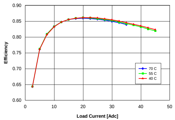
Fig. 1.2V.4: Efficiency vs. load current and ambient temperature for converter mounted vertically with V_{in} = 48\text{ V} and air flowing from pin 3 to pin 1 at a rate of 200 LFM (1.0 m/s).
