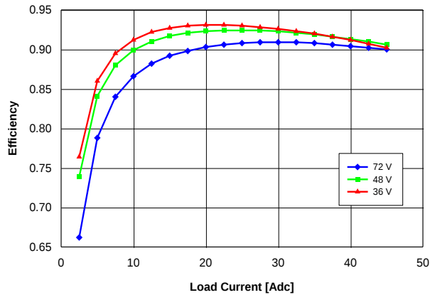
Fig. 3.3V.3: Efficiency vs. load current and input voltage for converter mounted vertically with air flowing from pin 3 to pin 1 at a rate of 300 LFM (1.5 m/s) and T_a = 25^\circ\text{C} .
