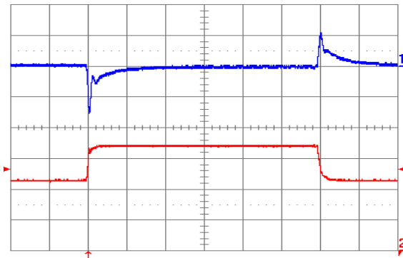
Fig. 1.5V.9: Output voltage response to load current step-change (22.5 A – 33.75 A – 22.5 A) at V_{in} = 48\text{ V} . Top trace: output voltage (100 mV/div.). Bottom trace: load current (10 A/div.). Current slew rate: 1 A/ \mu\text{s} . C_o = 470\text{ }\mu\text{F} tantalum + 1 \mu\text{F} ceramic. Time scale: 0.2 ms/div.
