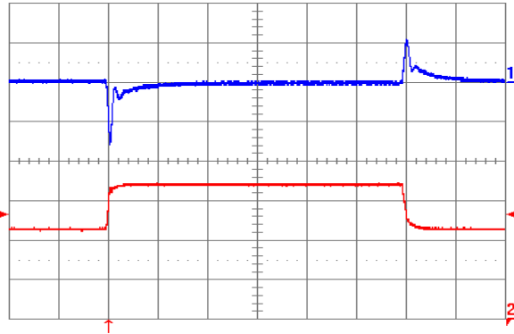
Fig. 1.2V.9: Output voltage response to load current step-change (22.5 A – 33.75 A – 22.5 A) at V_{in} = 48 V. Top trace: output voltage (20 mV/div.). Bottom trace: load current (10 A/div.). Current slew rate: 1 A/ \mu s. C_o = 470 \mu F tantalum + 1 \mu F ceramic. Time scale: 0.2 ms/div.
