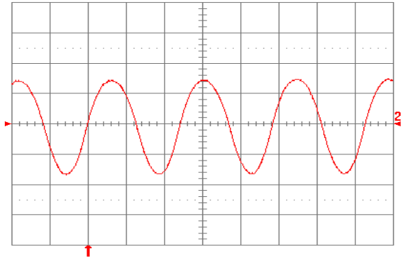
Fig. 2.0V.13: Input reflected ripple current, i_c (100 mA/div), measured at input terminals at full rated load current and V_{in} = 48 V. Refer to Fig. 2.0V.11 for test setup. Time scale: 1 \mu s/div.
