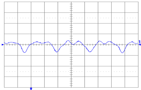
Fig. 1.5V.10: Output voltage ripple (20 mV/div.) at full rated load current into a resistive load with C_o = 10\text{ }\mu\text{F} tantalum + 1 \mu\text{F} ceramic and V_{in} = 48\text{ V} . Time scale: 1 \mu\text{s} /div.
