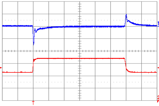
Fig. 2.5V.9: Output voltage response to load current step-change (22.5 A – 33.75 A – 22.5 A) at V_{in} = 48 V. Top trace: output voltage (100 mV/div.). Bottom trace: load current (10 A/div). Current slew rate: 1 A/ \mu s. C_o = 470 \mu F tantalum + 1 \mu F ceramic. Time scale: 0.2 ms/div.
