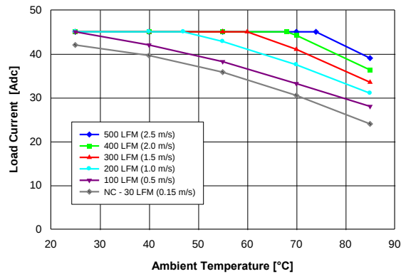
Fig. 2.0V.1: Available load current vs. ambient air temperature and airflow rates for QM48T45020 converter with B height pins mounted vertically with V_{in} = 48\text{ V} , air flowing from pin 3 to pin 1, and MOSFET temperature \leq 120\text{ }^{\circ}\text{C} . Note: NC – Natural convection
