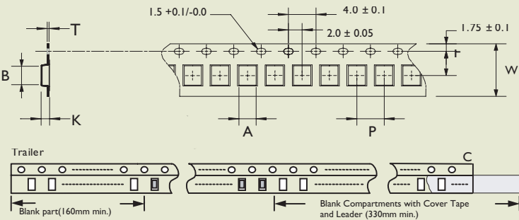
Tape Dimensions
