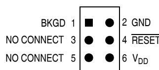
Figure 16-1. BDM Tool Connector
