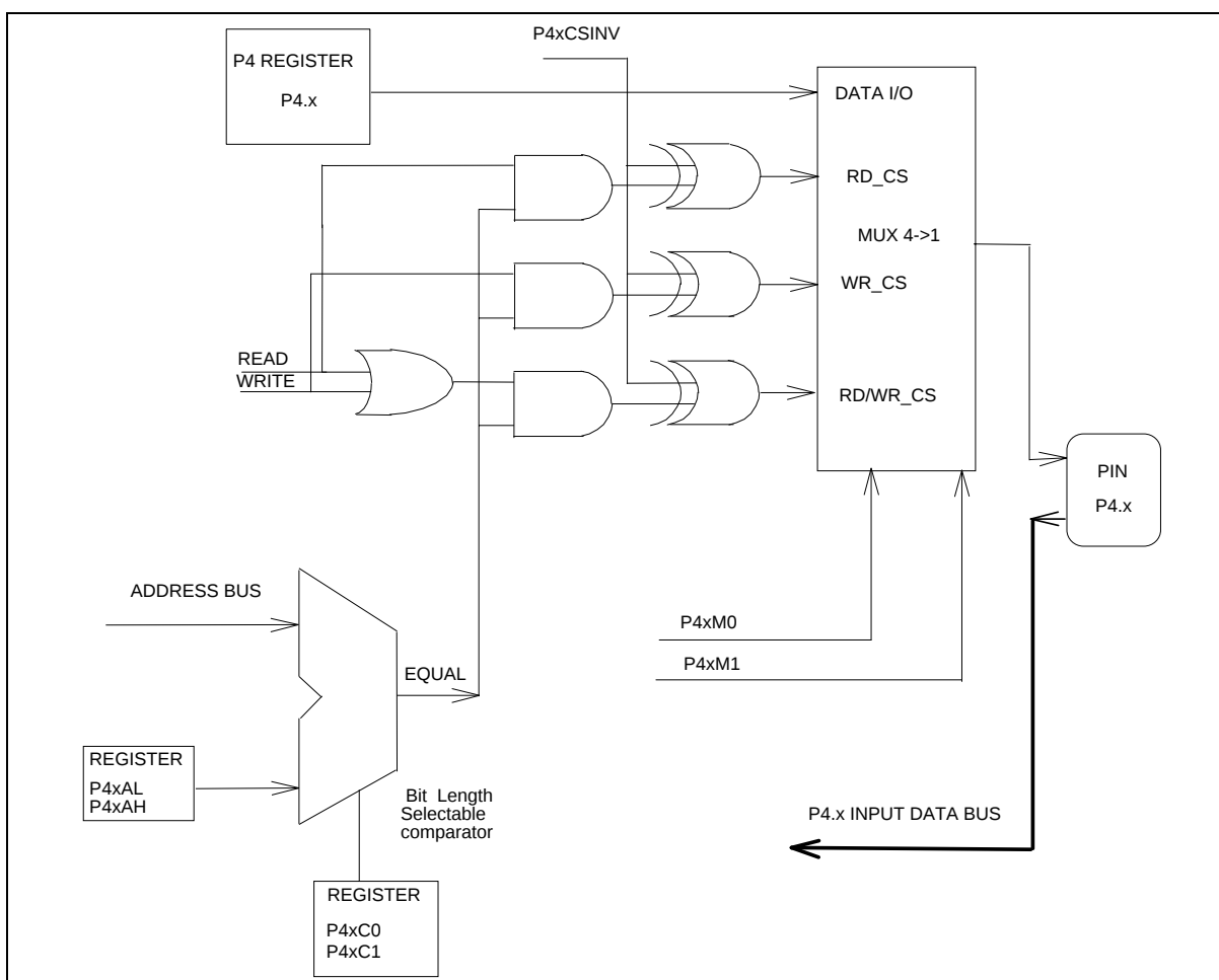
Figure 18-1 Port 4 Structure Diagram
