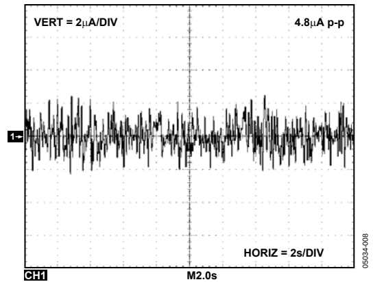
Figure 9. 0.1 Hz to 10 Hz Noise Plot ( V_{DD} = 3.6\text{ V} )
