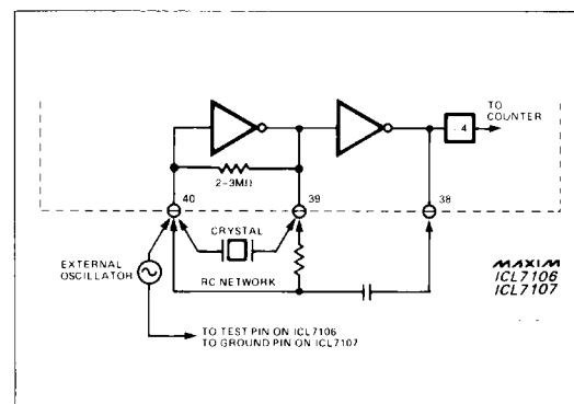
Figure 7. Clock Circuits
