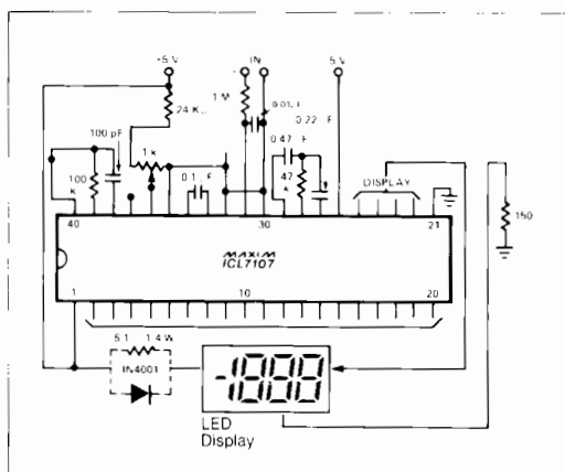
Figure 12. Diode or Resistor Limits Package Power Dissipation
