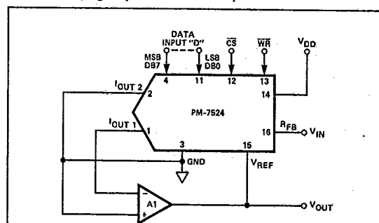
FIGURE 9: Divider (Digitally Controlled Gain)
