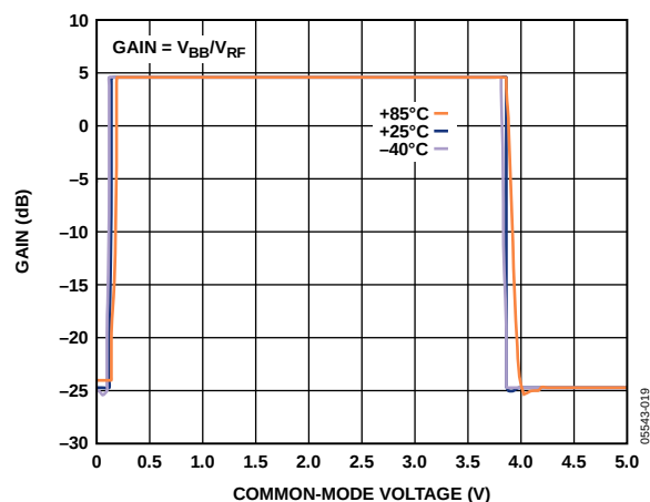
Figure 23. LO Common-Mode Range at Three Temperatures
