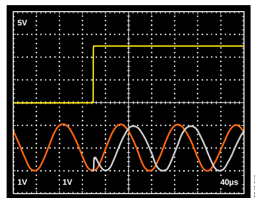
Figure 37. Phase Shifting Response—Channel 2 Leads Channel 1 by 90°, Top: Input to PH21, Select Code = 0100; Bottom (Red): Reference Channel 1 I_{OUT} ; Bottom (Gray): Channel 2 I_{OUT} Phase Shifted 90°, Channel 1 Reference Phase Code = 0000
