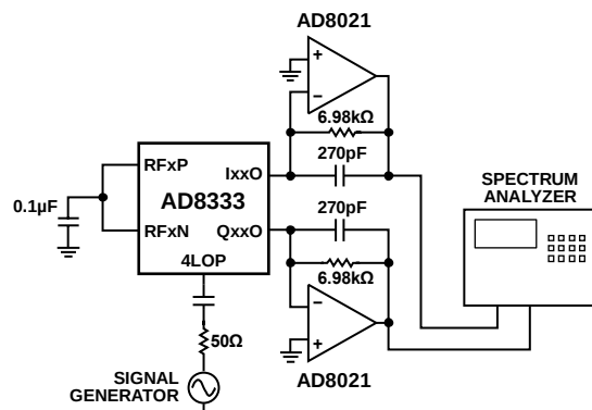
Figure 47. Noise Test Circuit
