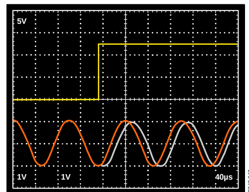
Figure 36. Phase Switching Response—Channel 2 Leads Channel 1 by 45°, Top: Input to PH21, Select Code = 0010; Bottom (Red): Reference Channel 1 I_{OUT} ; Bottom (Gray): Channel 2 I_{OUT} Phase Shifted 45°, Channel 1 Reference Phase Select Code = 0000
