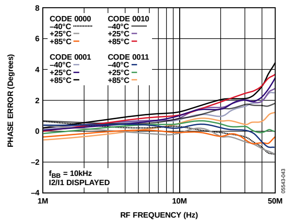
Figure 19. I2xO/I1xO or Q2xO/Q1xO Phase Error vs. RF Frequency, Baseband Frequency = 10 kHz, at Three Temperatures
