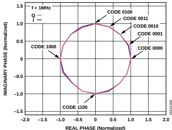
Figure 8. Normalized Vector Plot of Phase, Channel 2 with Respect to Channel 1; Channel 1 Is Fixed at 0^\circ ; Channel 2 Stepped 22.5^\circ/\text{Step} , All Codes Displayed
