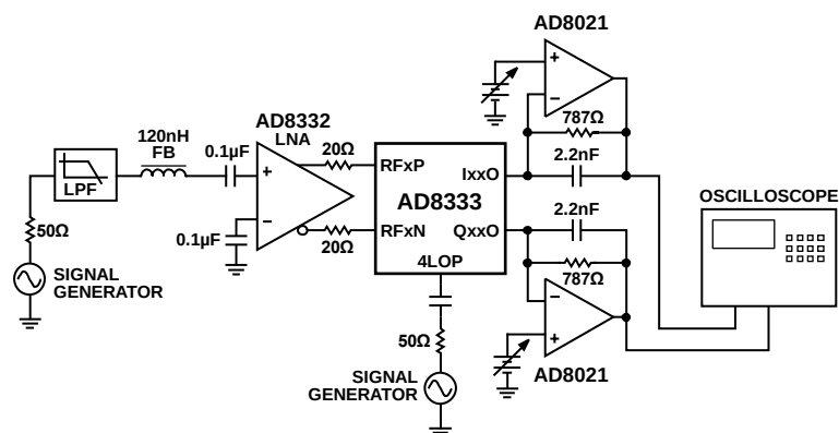
Figure 50. Output Compliance Range
