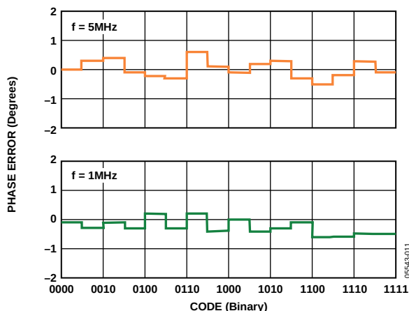
Figure 11. Phase Error of Channel 2 with Respect to Channel 1 vs. Code at 1 MHz and 5 MHz
