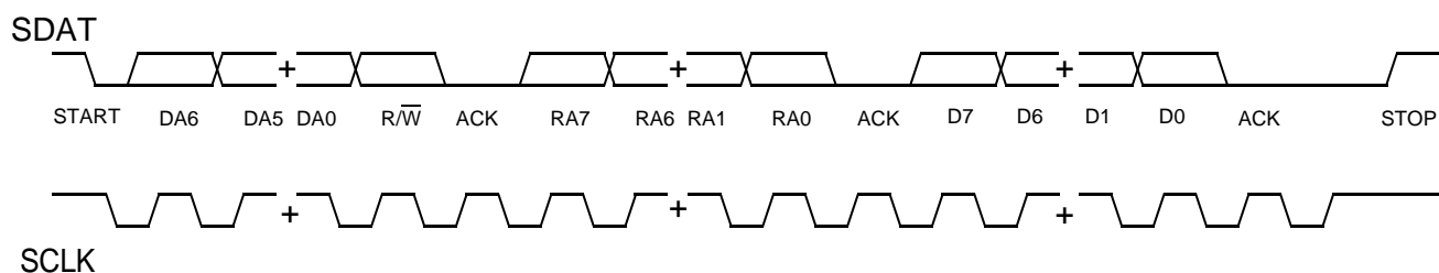
Figure 8. Frame Format (Device Address, \overline{R/\overline{W}} , Register Address, Register Data)
