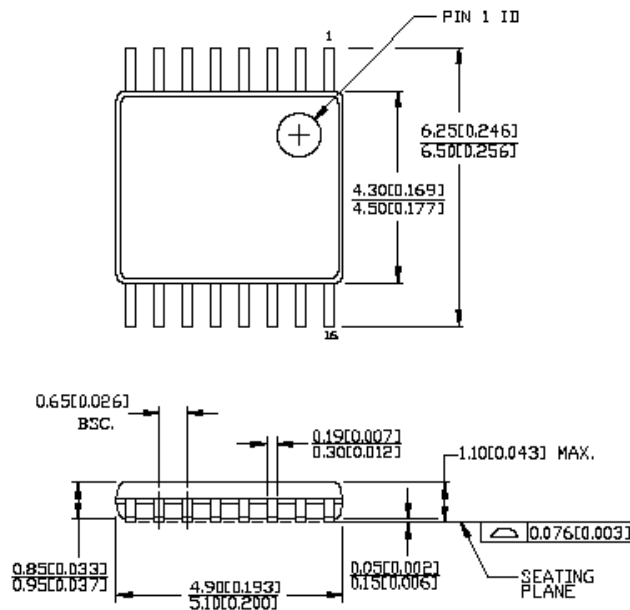
Figure 12. 16-Pin TSSOP 4.40 mm Body Z16.173
