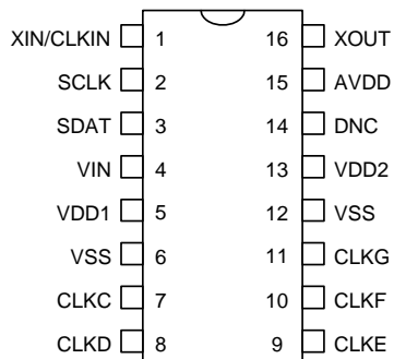
Figure 1. Pin Configuration – CY24488 16-Pin TSSOP
