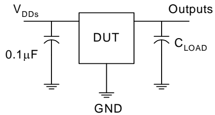
Figure 9. Test and Measurement Diagram
