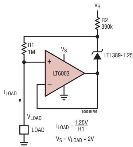
Figure 5. Precision 1.25μA Current Source
