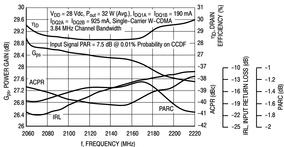
Figure 6. Output Peak-to-Average Ratio Compression (PARC) versus Broadband Performance @ P_{out} = 32 \text{ Watts Avg.}
