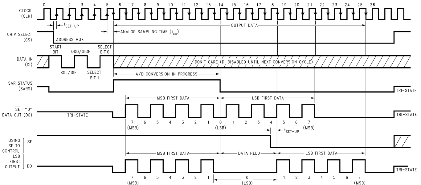
Figure 18. ADC08038 Timing
