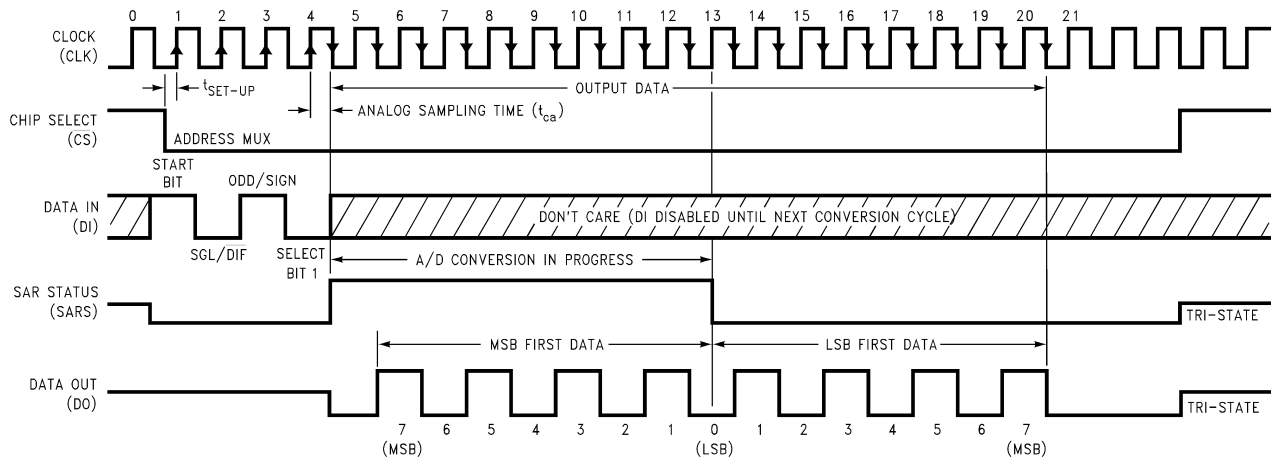
Figure 18. ADC08038 Timing
