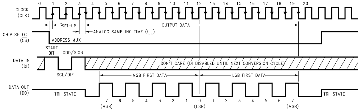
Figure 17. ADC08034 Timing
