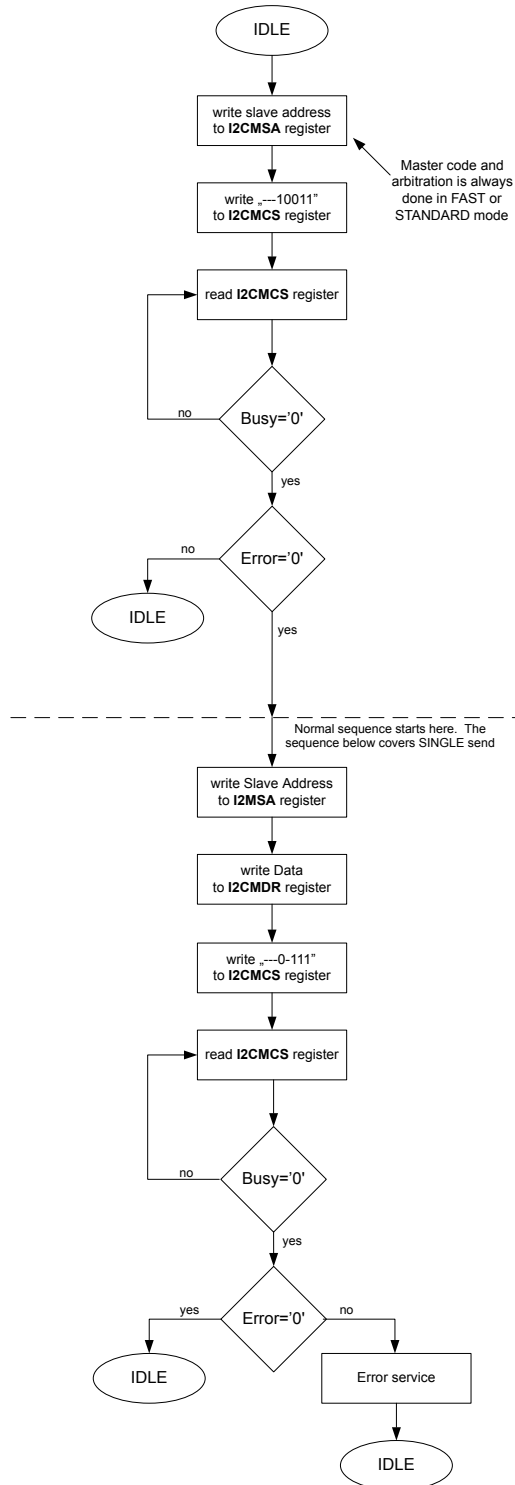
Figure 15-14. Standard High Speed Mode Master Transmit
