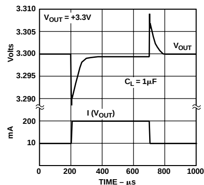
Figure 13. Load Transient for 10 mA to 200 mA Pulse
