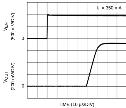
0.7-V Option
