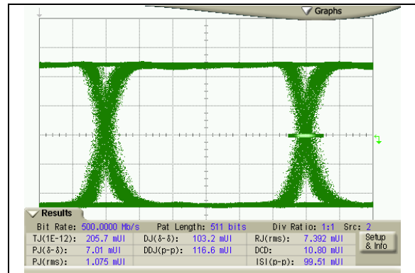
FIGURE B-11: 70M CAT5E - RX ONLY
