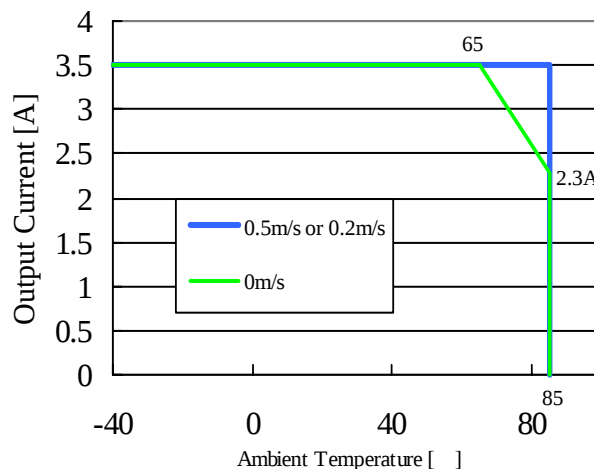
MPD6D102S ( V_o=1.2\text{V} )
