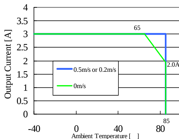
MPD6D104S ( V_o=1.8\text{V} )
