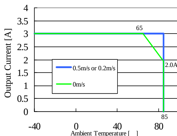
MPD6D106S ( V_o=2.5\text{V} )
