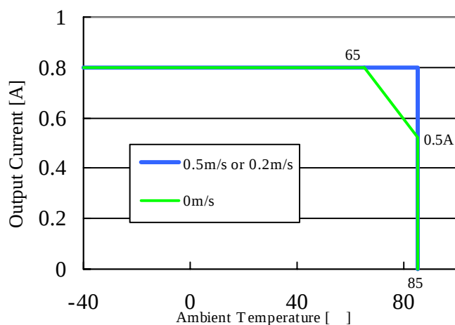
MPD6D101S ( V_o=12\text{V} )
