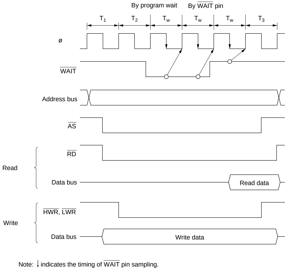
Figure 6-14 Example of Wait State Insertion Timing
