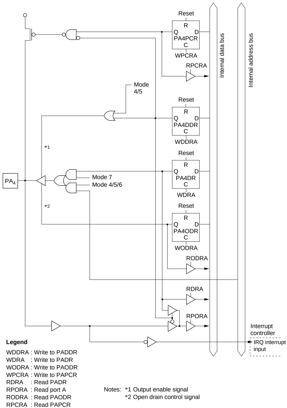
Figure C-7 (b) Port A Block Diagram (Pin PA 4 )
