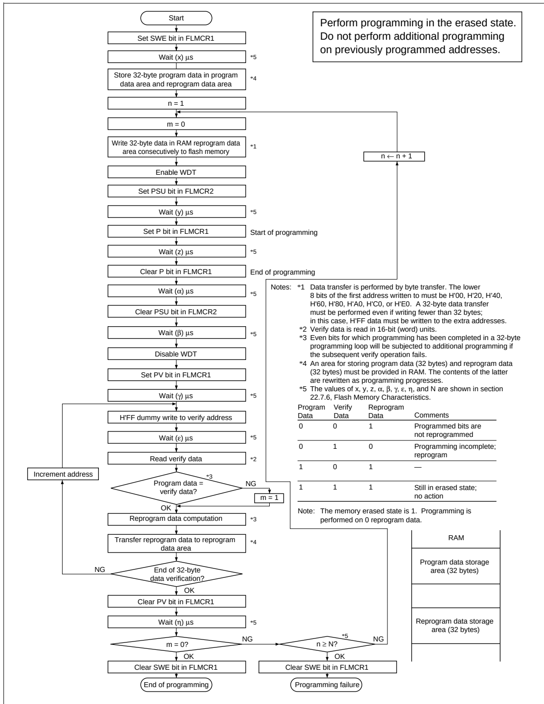
Figure 19-19 Program/Program-Verify Flowchart
