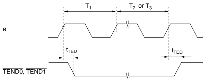
Figure 22-84 DMAC \overline{TEND} Output Timing
