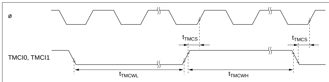
Figure 22-59 8-Bit Timer Clock Input Timing
