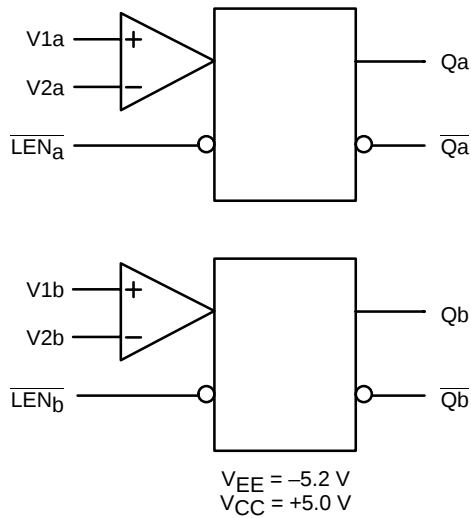
Figure 2. Logic Diagram
