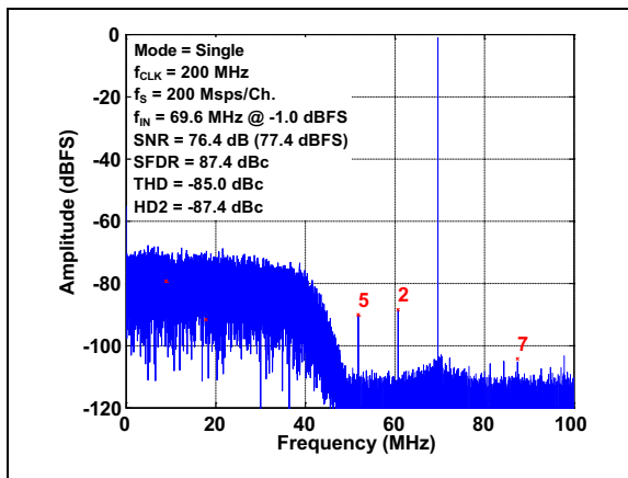
FIGURE 3-14: FFT for 69.6 MHz Input Signal with NSR enabled: NSR = 20, f_S = 200 Msps/Ch., A_{IN} = -1 dBFS.
