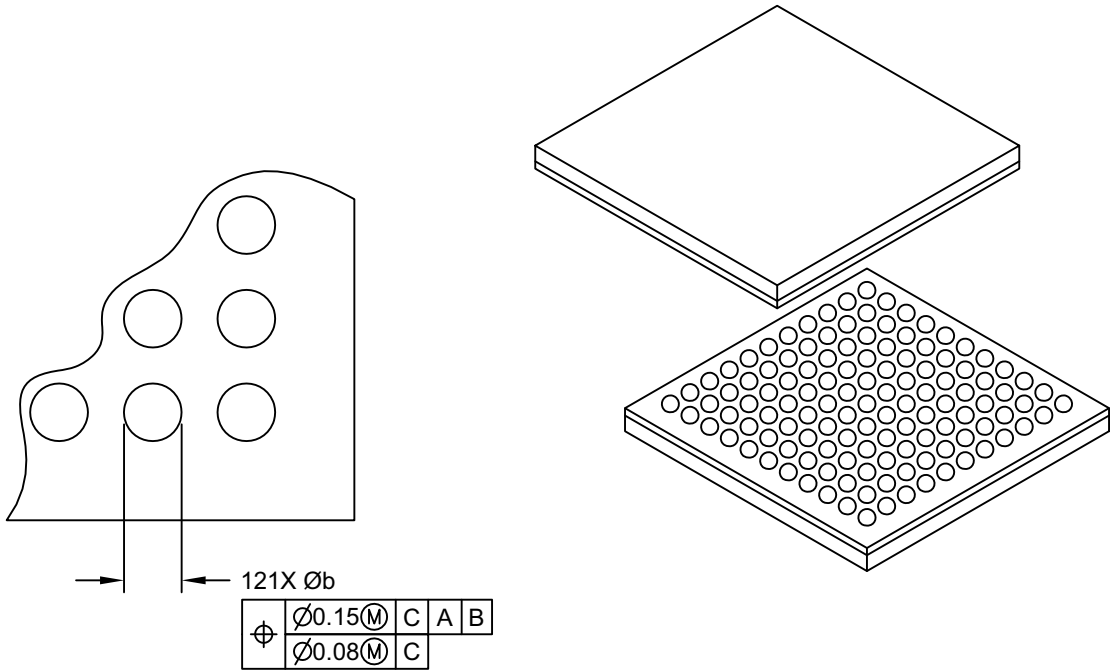
DETAIL A
