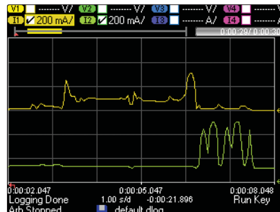
Figure 6. In Datalog View, you can log data on multiple traces. Here, the current flowing out of output 1 and output 2 are captured over 30 seconds
