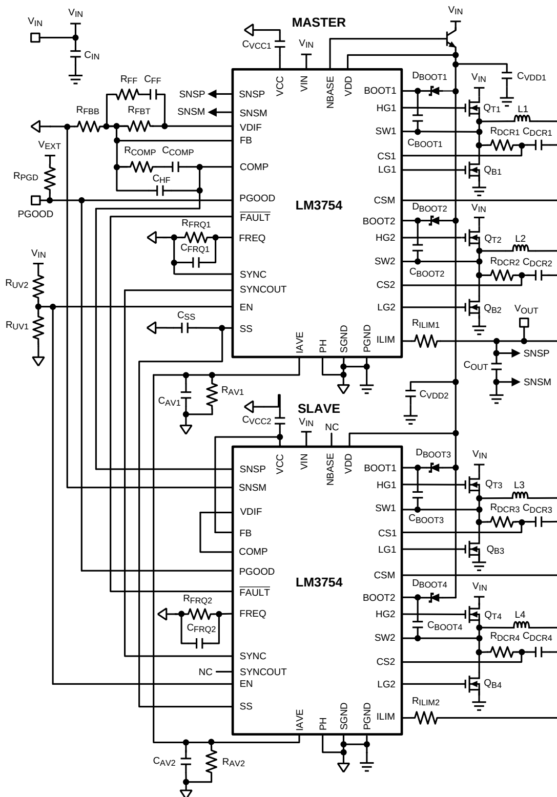
Figure 29. Typical Application
