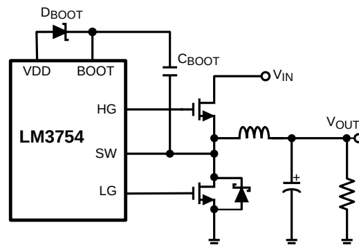
Figure 18. Bootstrap Circuit
