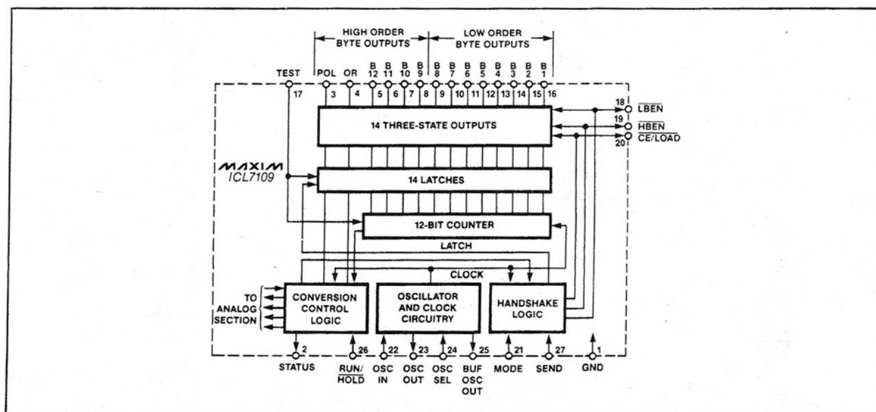
Figure 4. Digital Section
