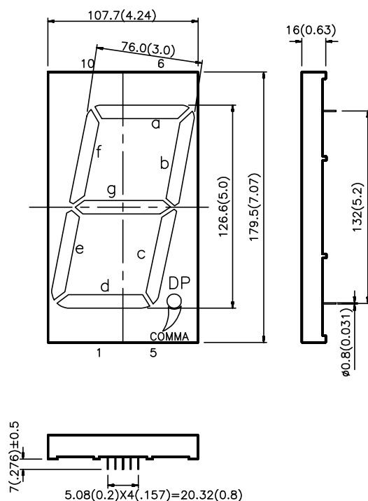
Package Dimensions
