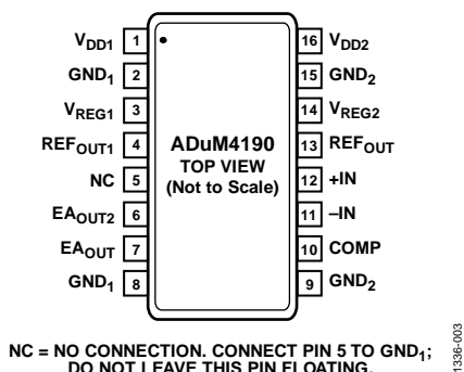
Figure 3. Pin Configuration
