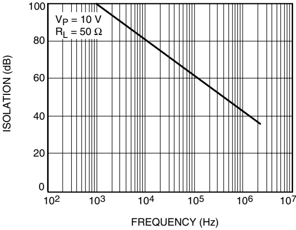
Figure 8. Output Isolation
