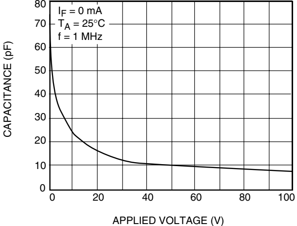
Figure 3. Switch Capacitance vs. Applied Voltage
