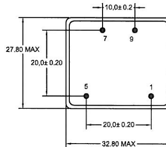
Single output
