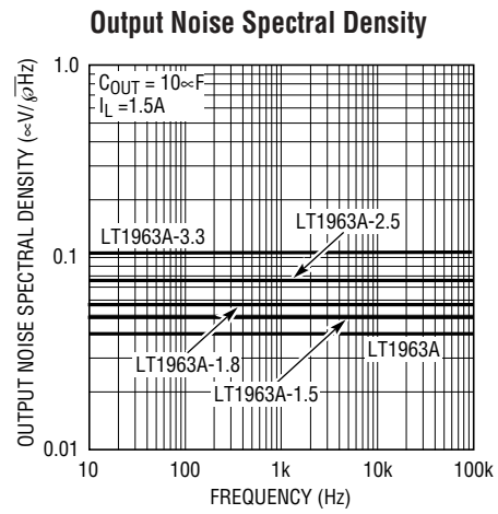
LT1963A-3.3 10Hz to 100kHz Output Noise
