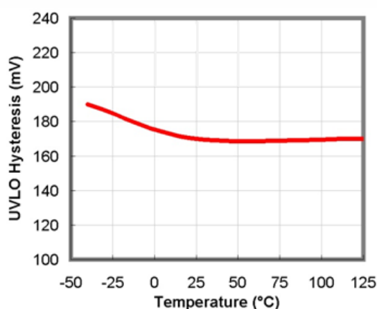
Figure 15. UVLO Hysteresis vs. Temperature
