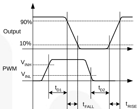
Figure 7. DIM Pin
