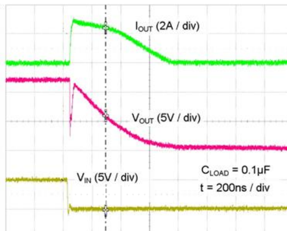
Figure 25. Quasi-Static Sink Current with V_{DD}=12\text{ V}
