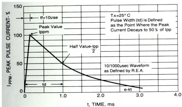
FIG.3-PULSE WAVEFORM
