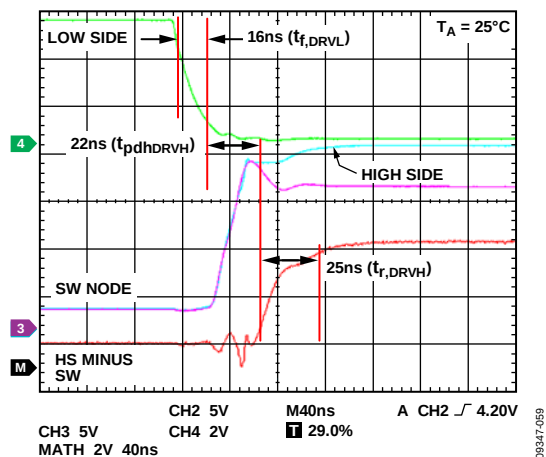
Figure 59. Upper Side Driver Rising and Lower Side Falling Edge Waveforms ( C_{IN} = 4.3 \text{ nF} (Upper Side/Lower Side MOSFET), Q_{TOTAL} = 27 \text{ nC} ( V_{GS} = 4.4 \text{ V} (Q1), V_{GS} = 5 \text{ V} (Q3))
