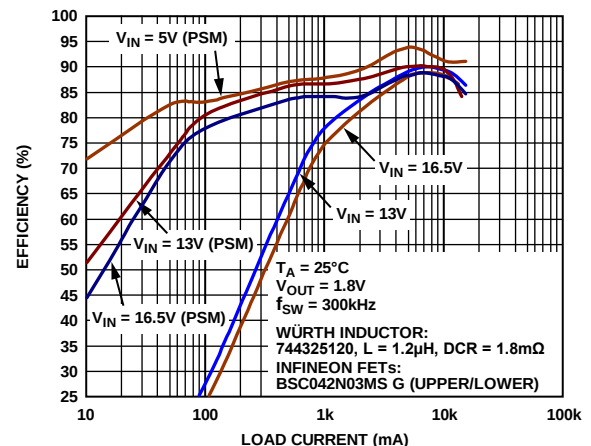
Figure 2. ADP1874/ADP1875 Efficiency vs. Load Current ( V_{OUT} = 1.8 V, 300 kHz)
