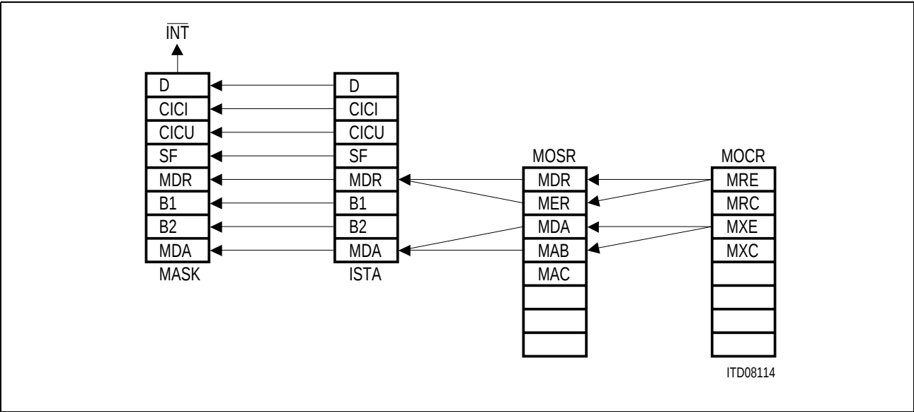
Figure 90 Interrupt Structure
