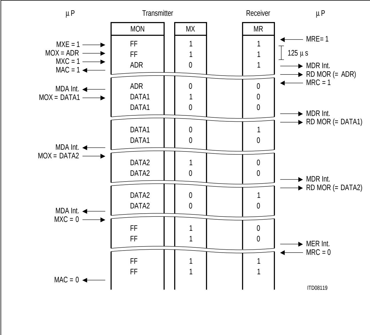
Figure 43 Monitor Channel Protocol
