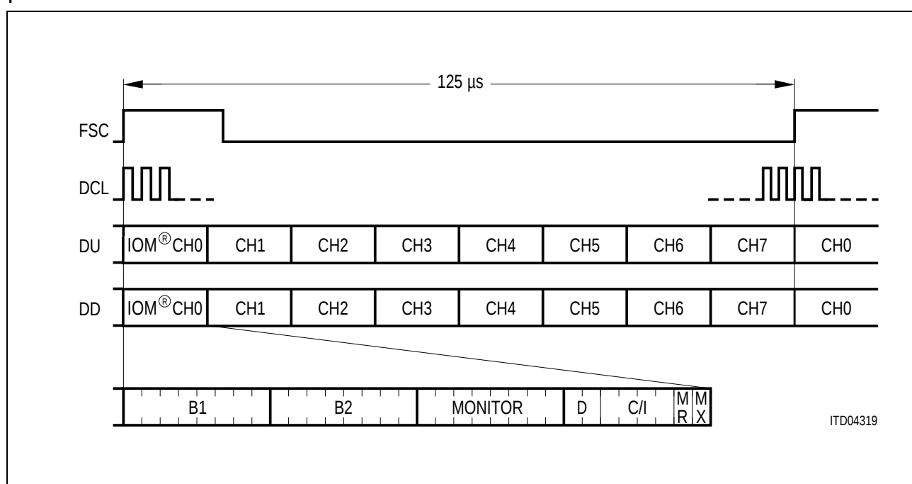
Figure 25 Multiplexed Frame Structure of the IOM ® -2 Interface
