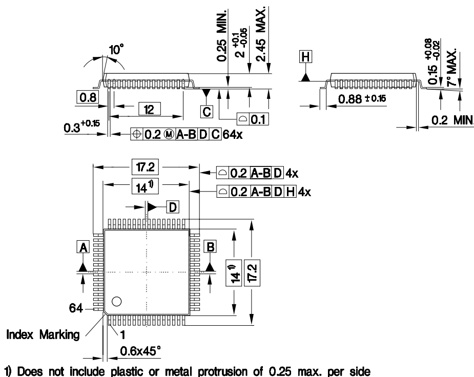
Figure 126 Package Outline for M-QFP-64
