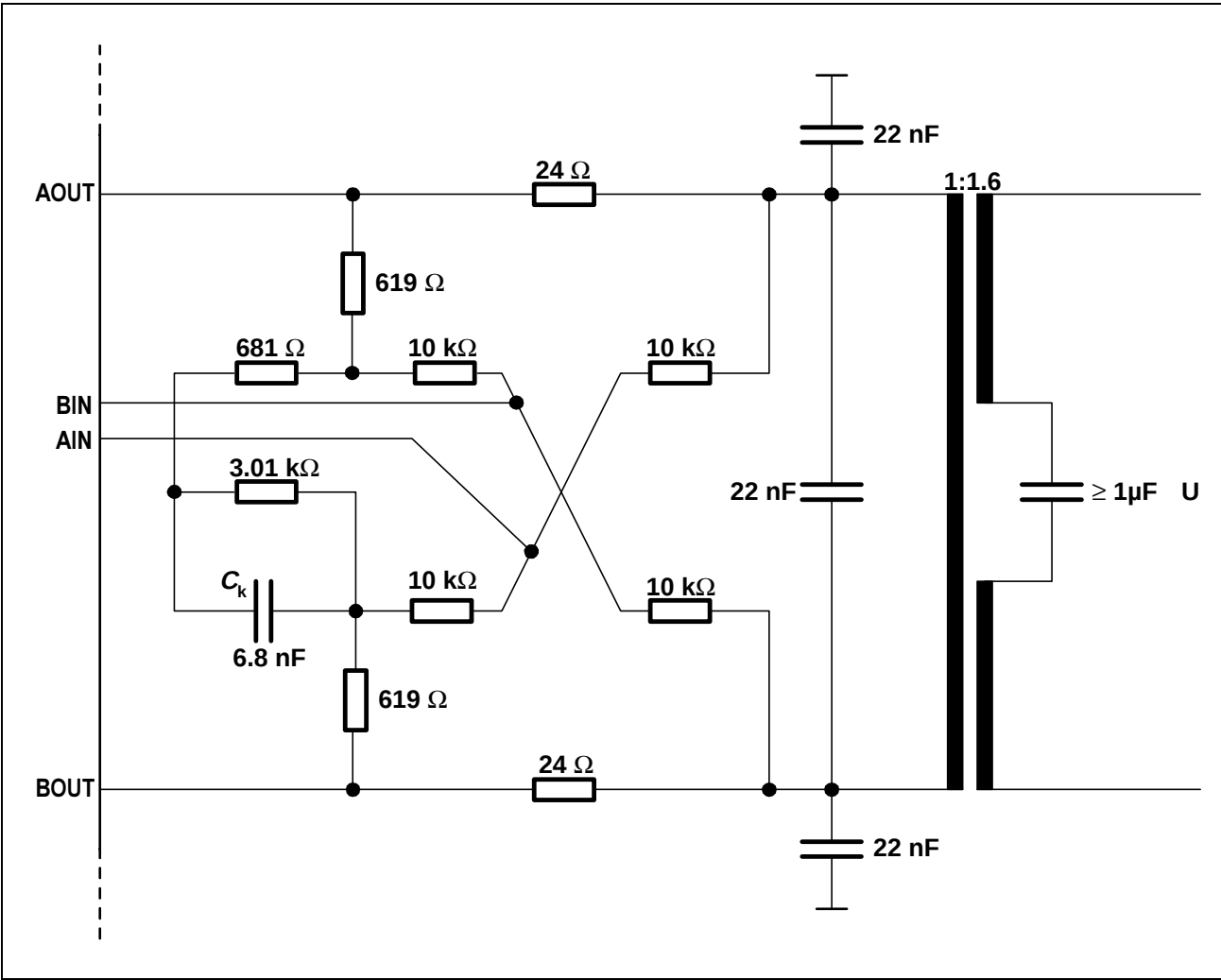
Figure 93 U-Interface Hybrid Circuit
