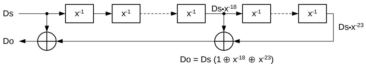
Receiver Descrambler for all LT Modes and for Loop-Back 3 in all NT Modes
