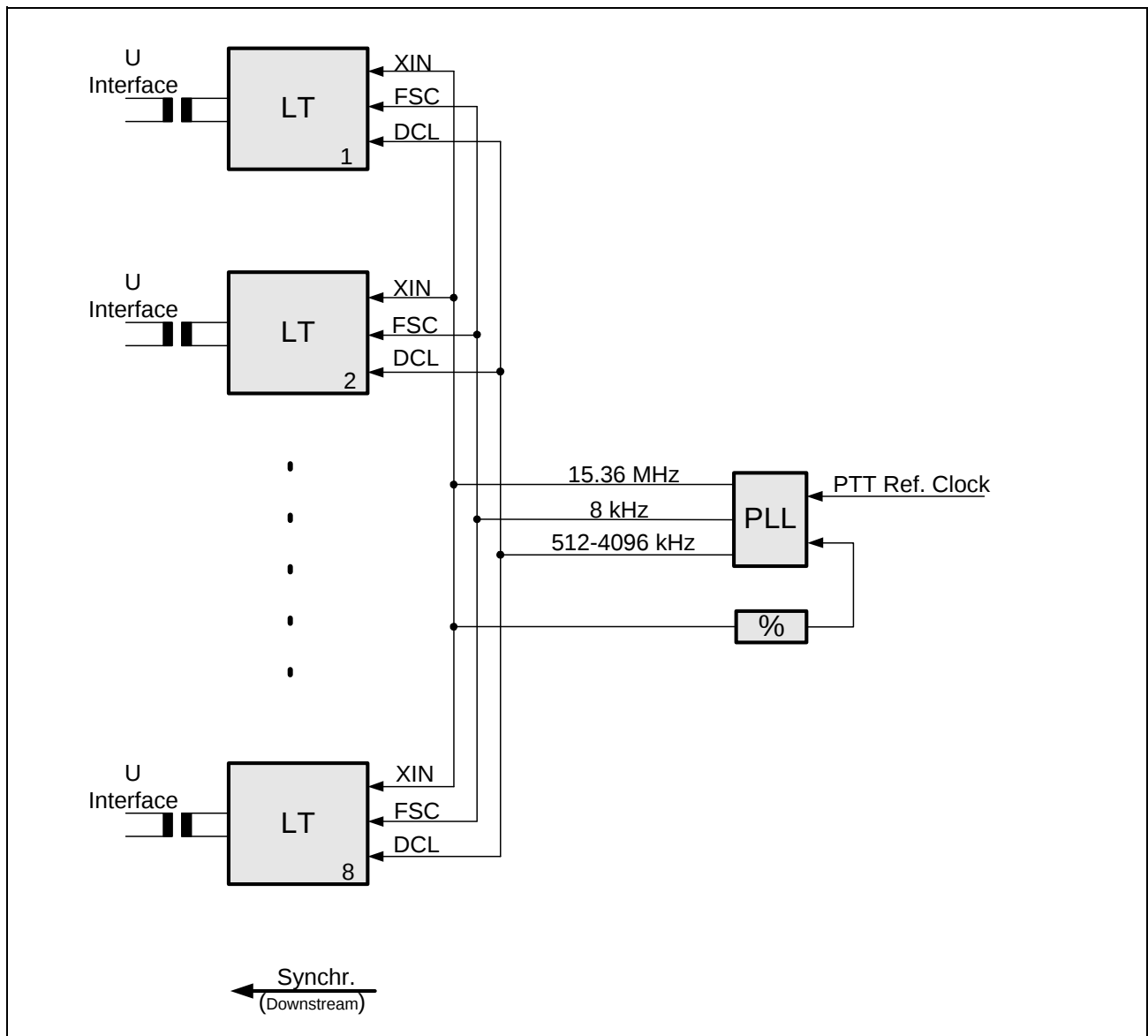
Figure 32 Clock Generation for LT Mode
