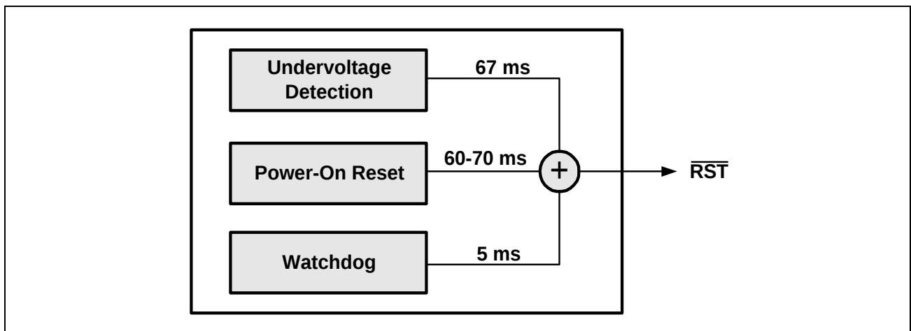
Figure 38 Reset Sources
