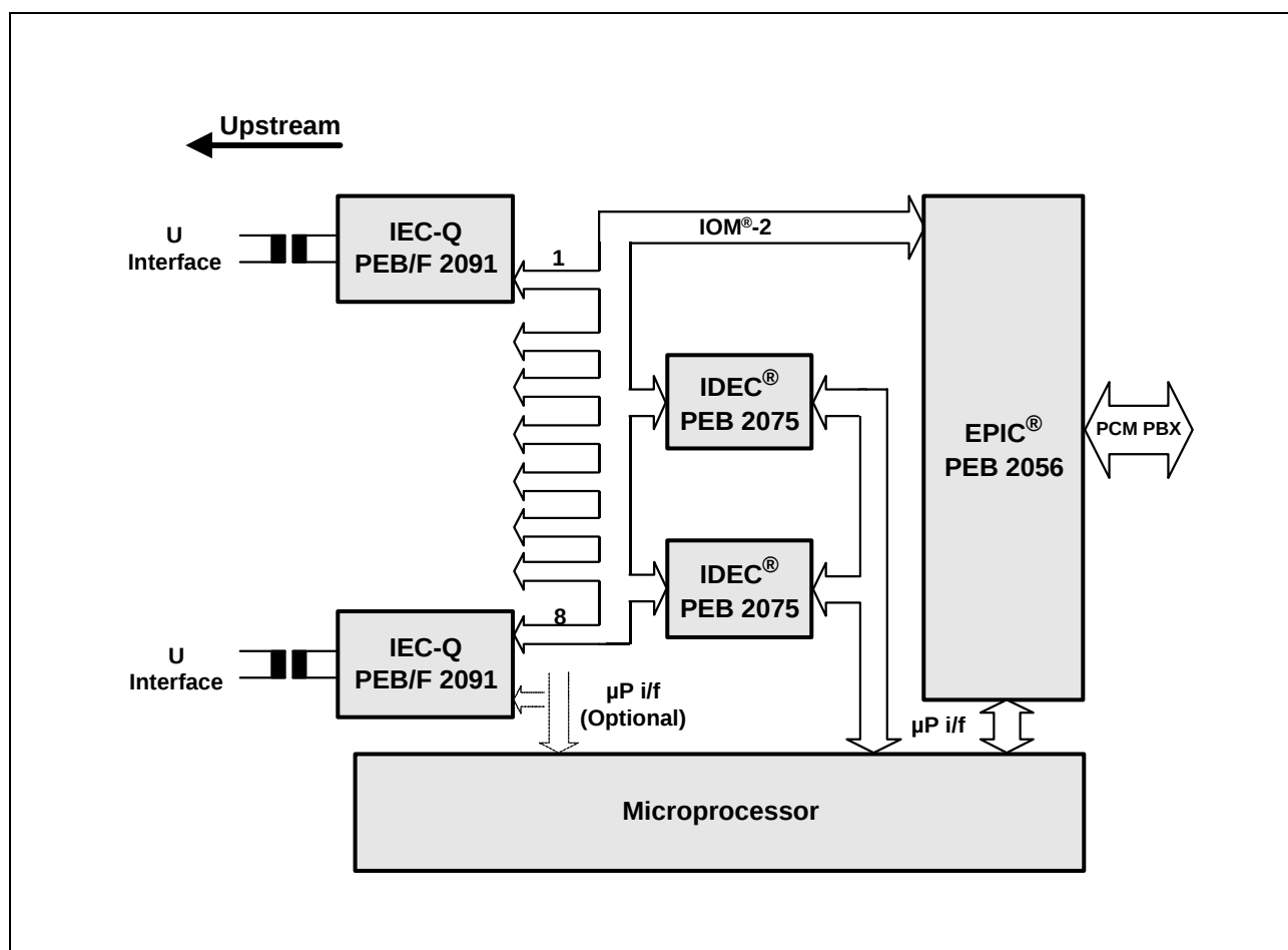
Figure 10 NT-PBX Application
