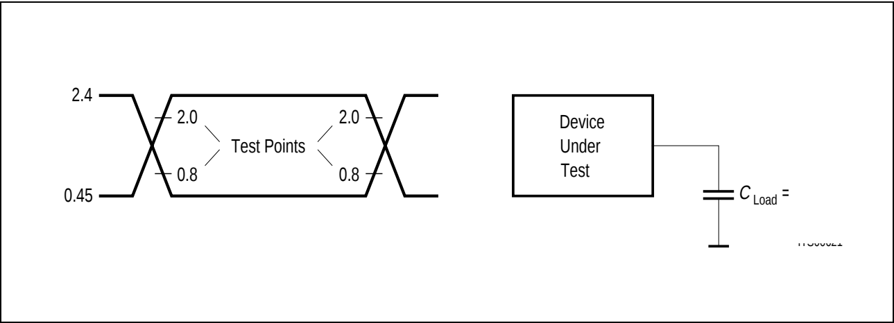
Figure 103 Input/Output Wave form for AC Tests
