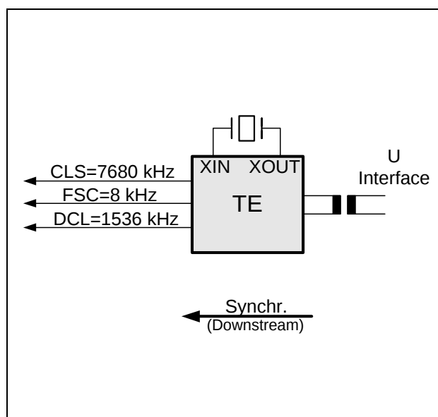
Figure 33 Clocks in TE Mode
