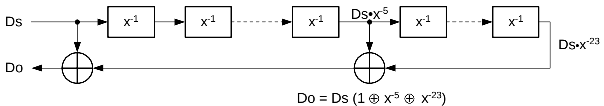
Receiver Descrambler in NT, NT-PBX and TE Mode without Loop-Back 3
