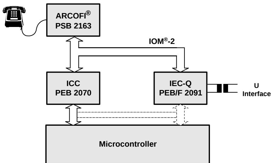
Figure 8 TE Application
