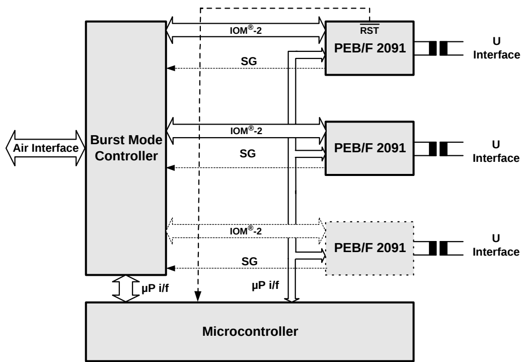
Figure 7 Architecture of the Wireless Local Loop Base Station
