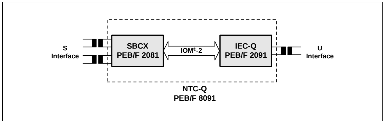
Figure 12 NT1 Application
