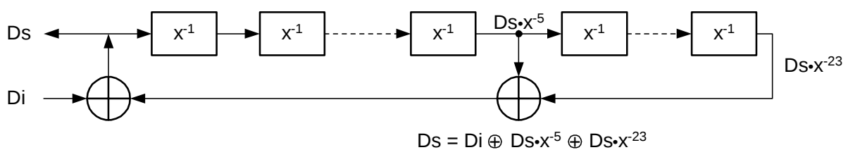
Transmitter Scrambler for all LT Modes and for Loop-Back 3 in all NT Modes
