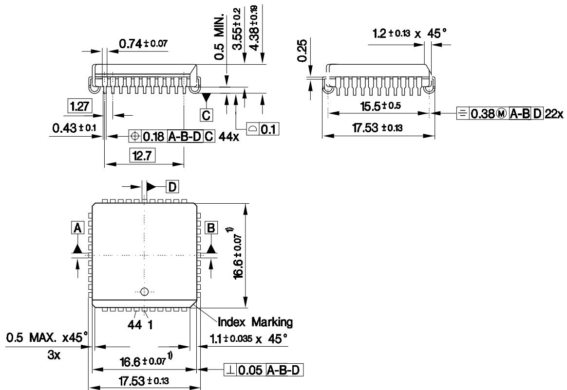
Figure 125 Package Outline for P-LCC-44
