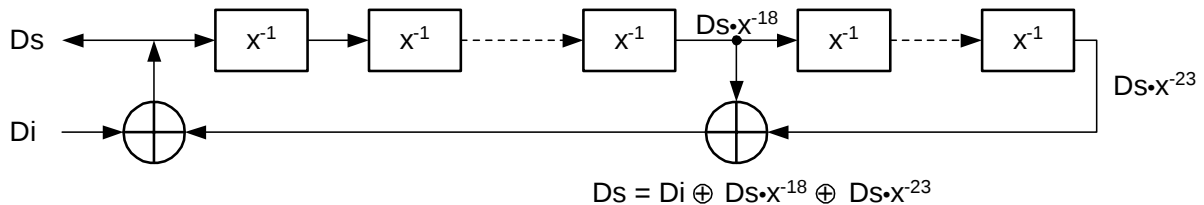
Transmitter Scrambler in NT, NT-PBX and TE Mode without Loop-Back 3
