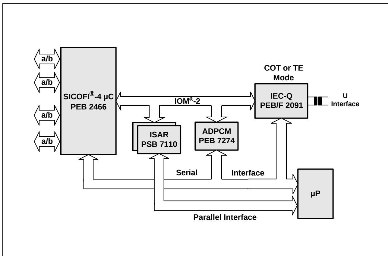
Figure 5 PCM 4 Application
