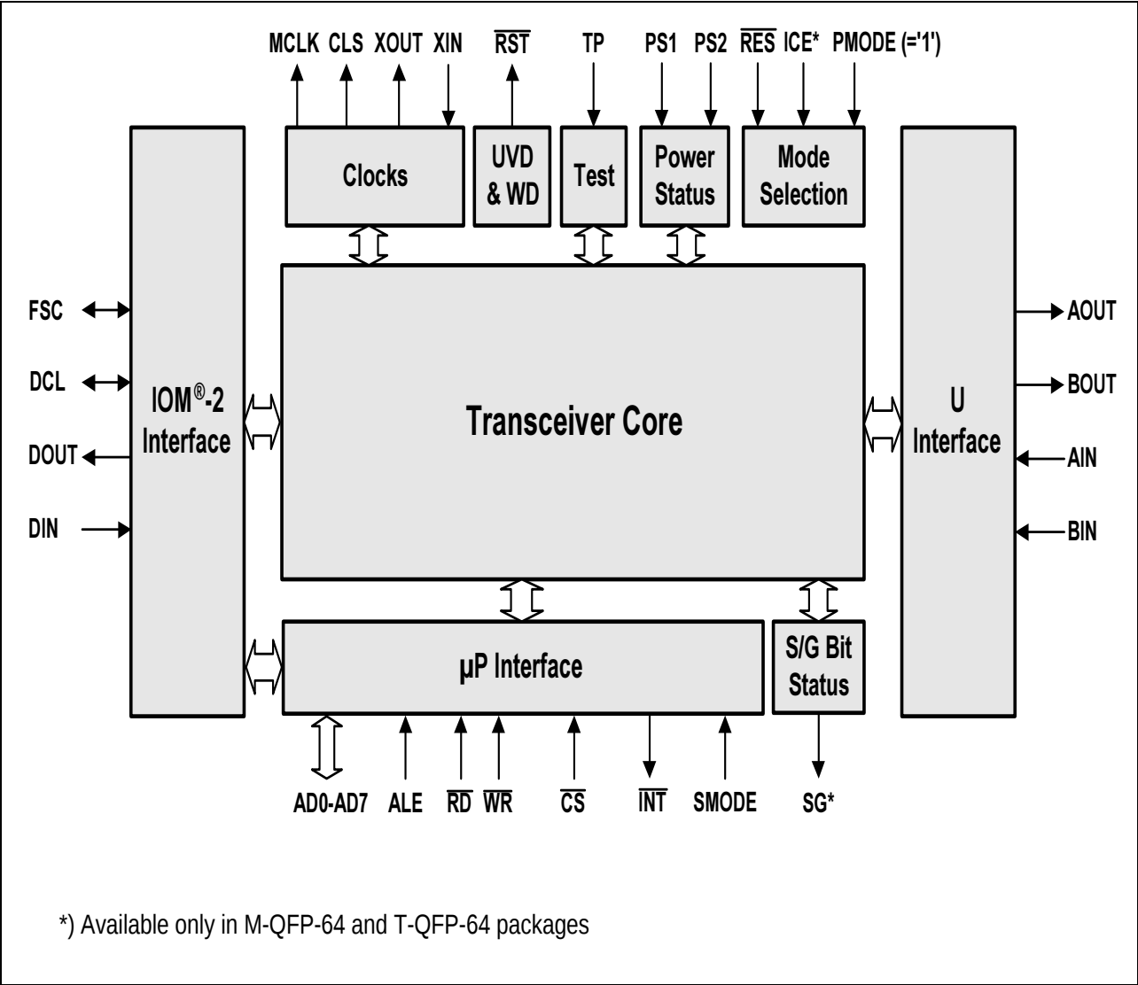
Figure 16 Device Architecture in µP Mode
