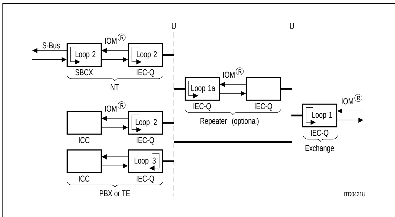
Figure 80 Test Loop-Backs Supported by the IEC-Q
