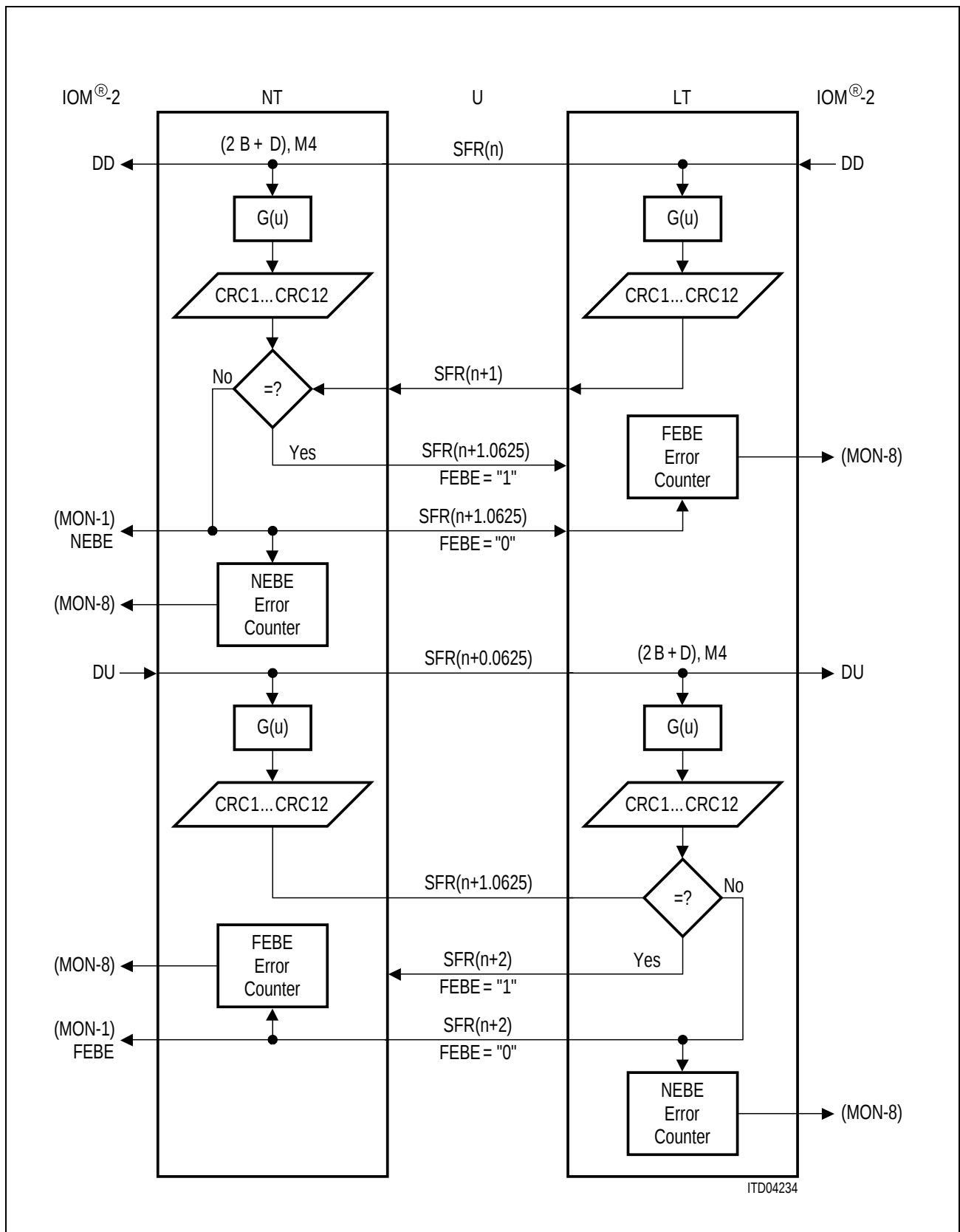
Figure 79 CRC Violation Indications
